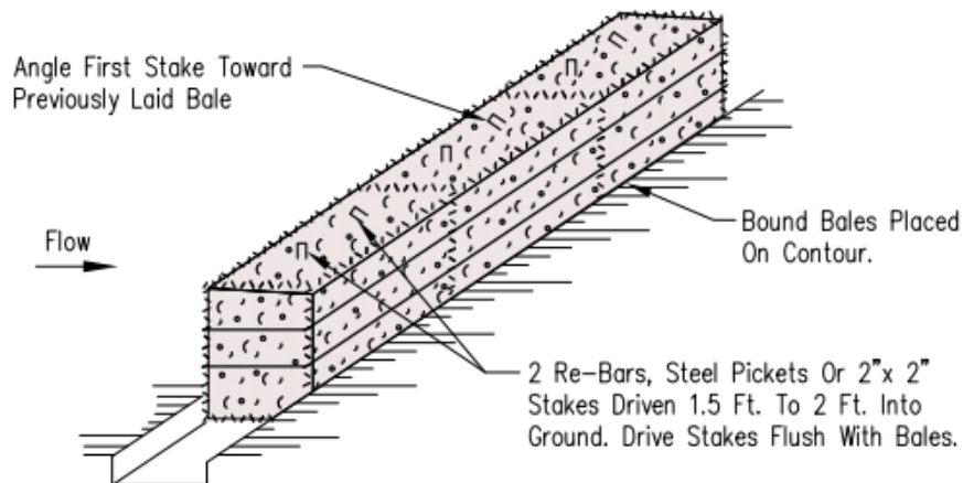
ANCHORING DETAIL
