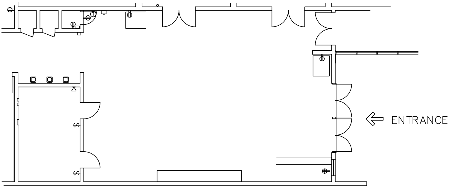
PETALUMA LOBBY 31' X 45'
