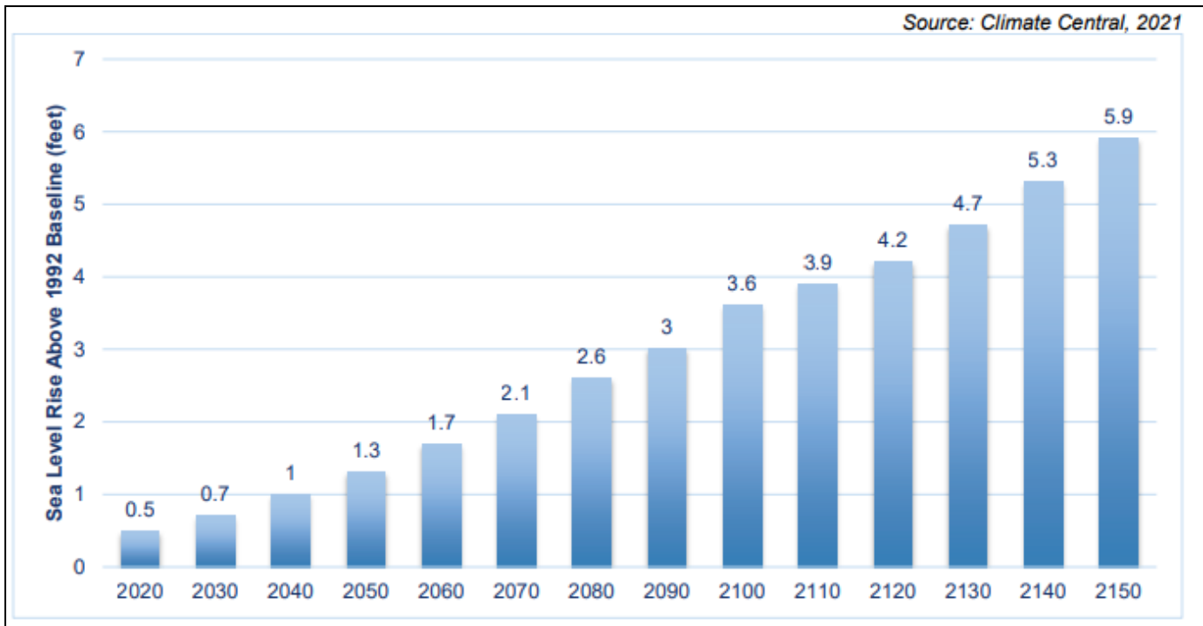
Figure 14-2. Medium Projection for Sonoma County Sea Level Rise Above 1992 Baseline
