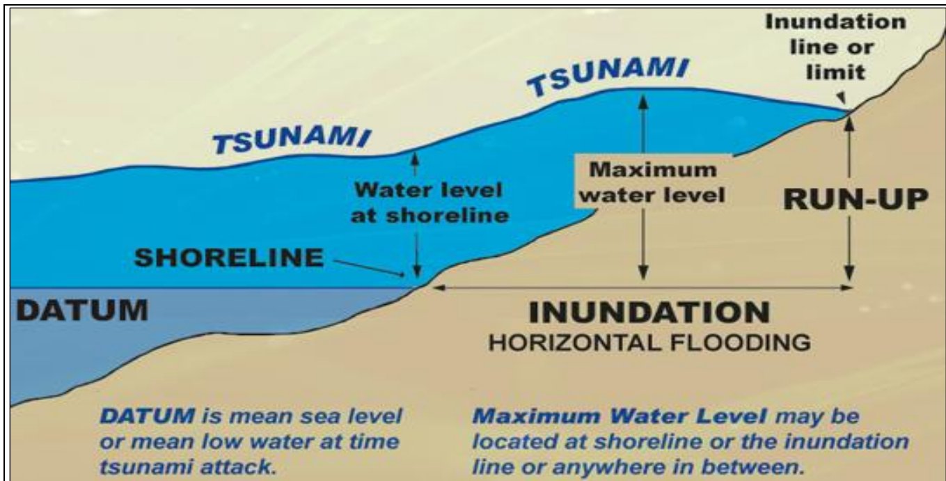
Figure 15-1. Run-up Distance and Height In Relation to the Datum and Shoreline
