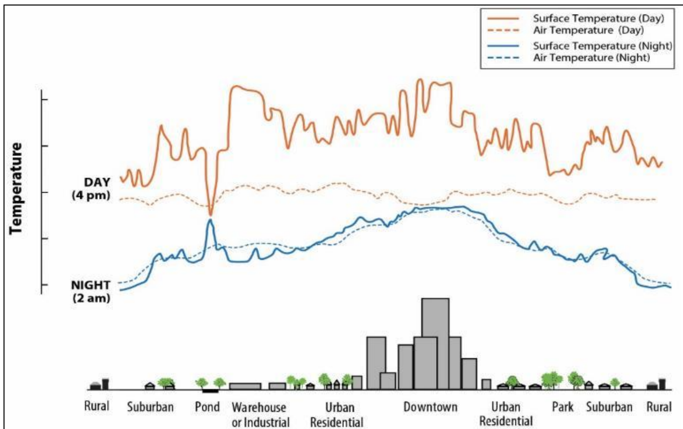
Figure 10-1. Heat Island Effect Diagram
